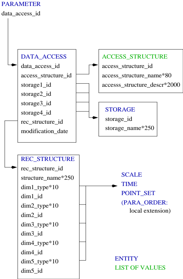
Figure 3. Data Access Modul
